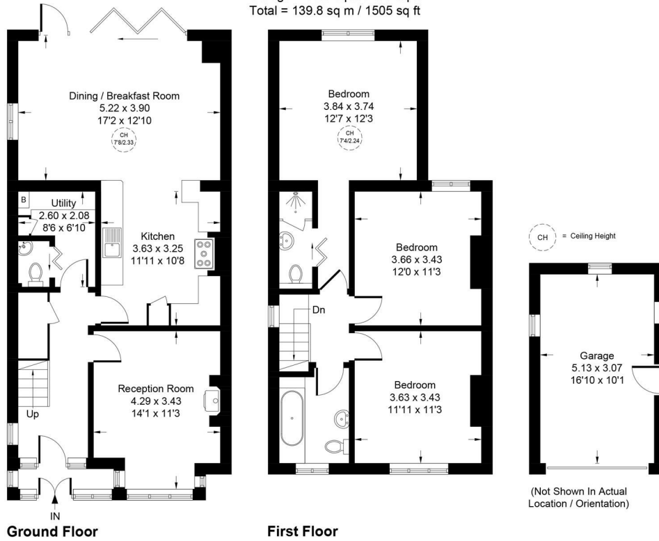
Floor plan produced in accordance with RICS Property Measurement Standards incorporating International Property Measurement Standards (IPMS2 Residential). Produced for Burton Matthews Estate Agents by DRAW EASY PLANS LIMITED
